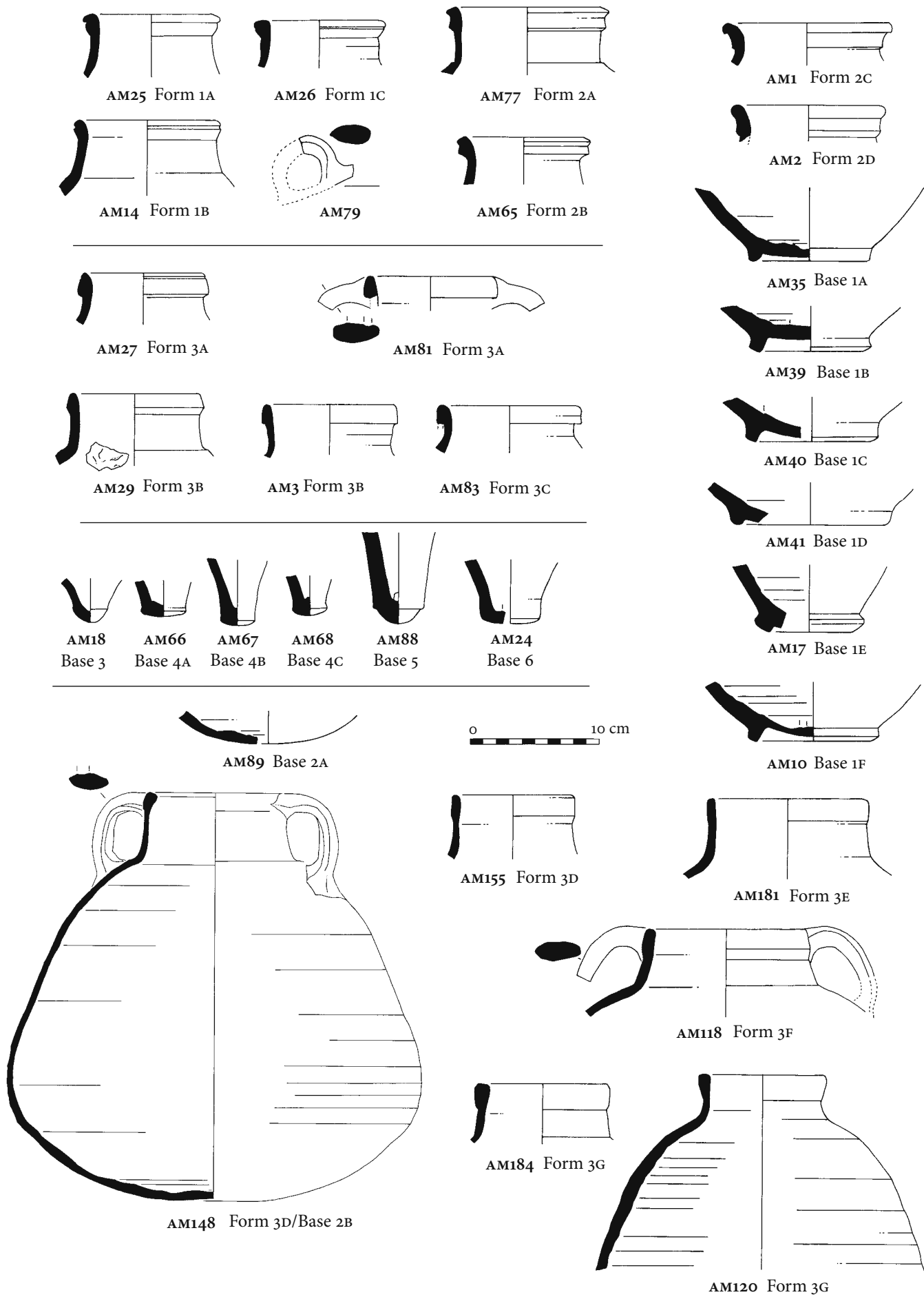
Plate 43. Typology. Form 1 to Form 3. Late Augustan/Tiberian to mid-third century A.D.
