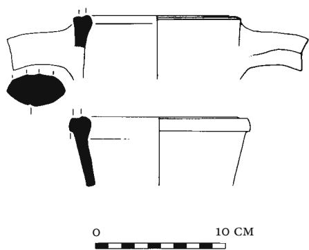
a-b) Jabbul Plain Survey (Aleppo): Site JP 99, Form 16A (top) and Form 15C
