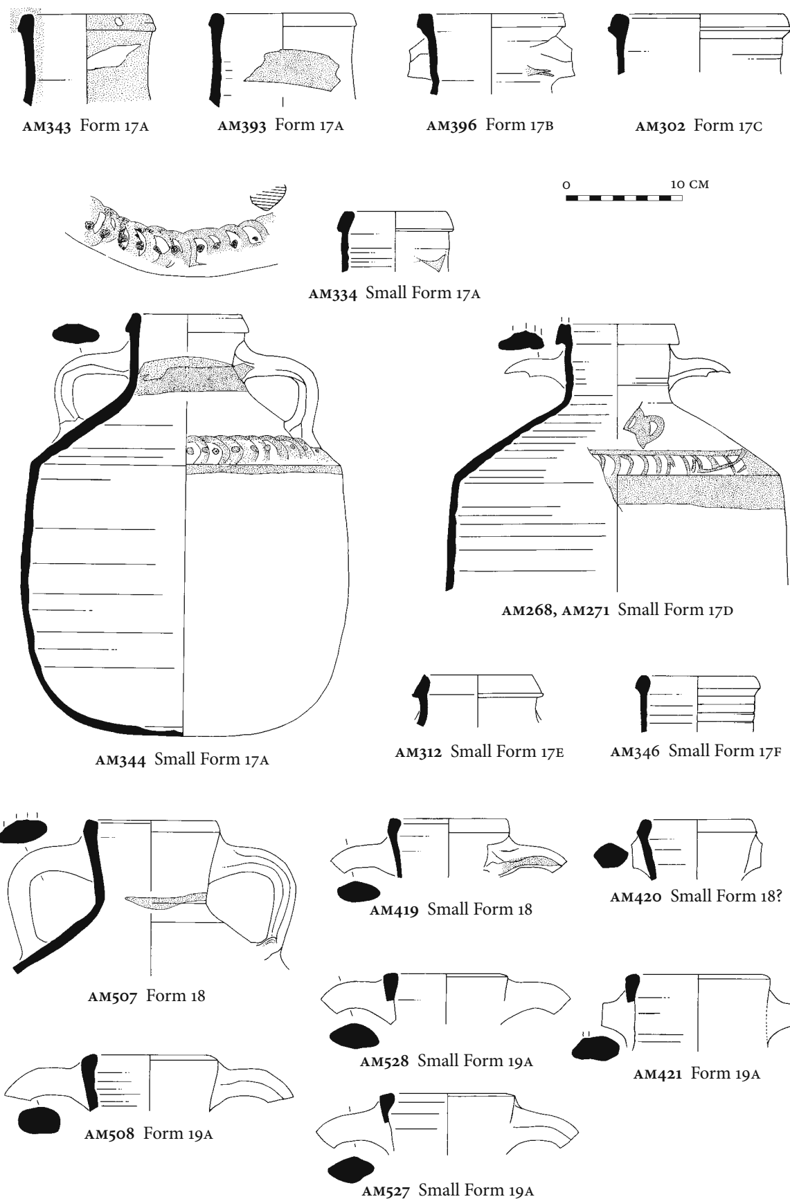
Plate 48. Typology. Form 17 to Form 19 (Syrian Fabric 13). Early seventh century A.D.
