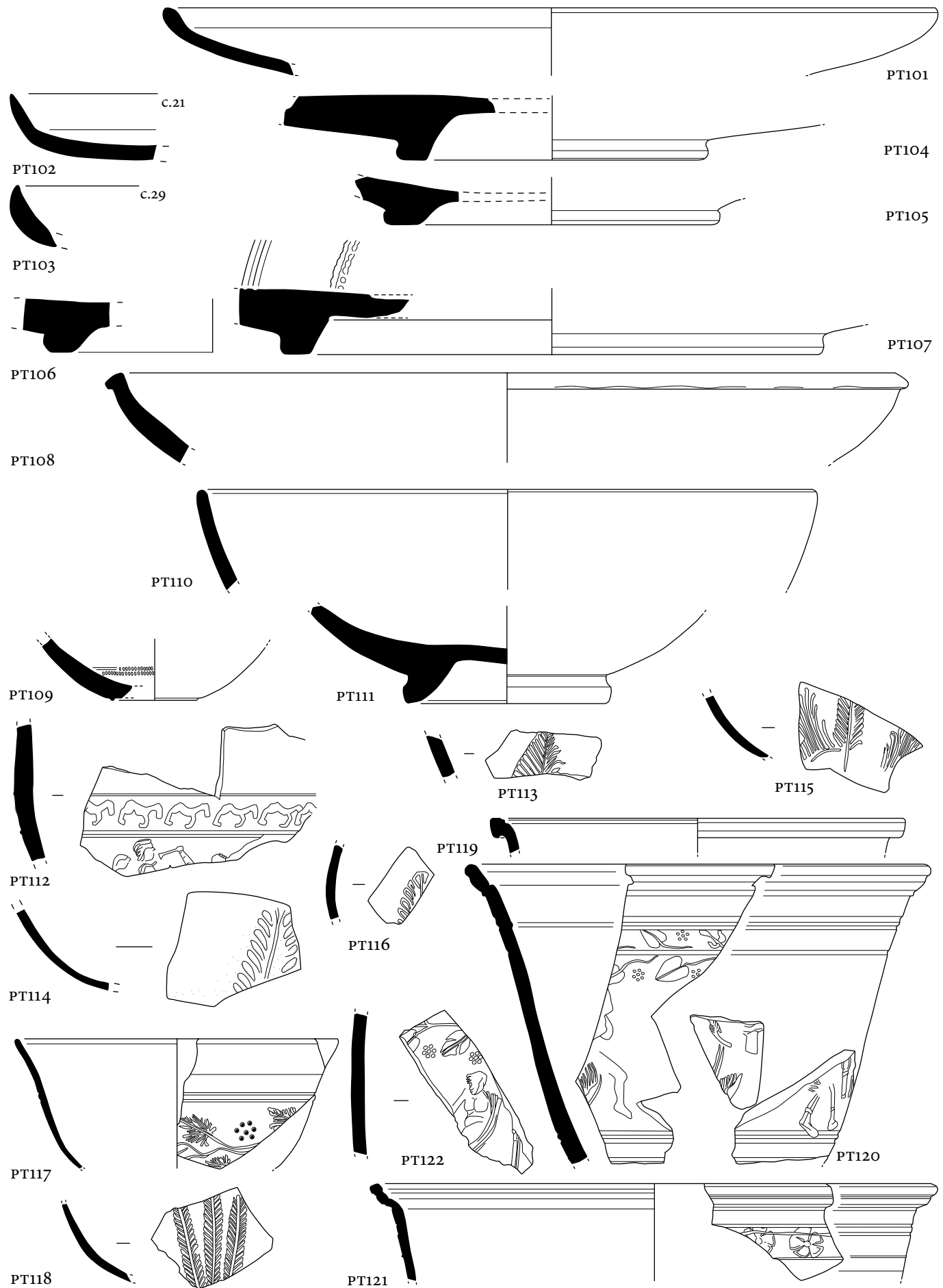
Plate 8. Group B. Eastern Sigillata A (PT101–122). Scale 1:2.
