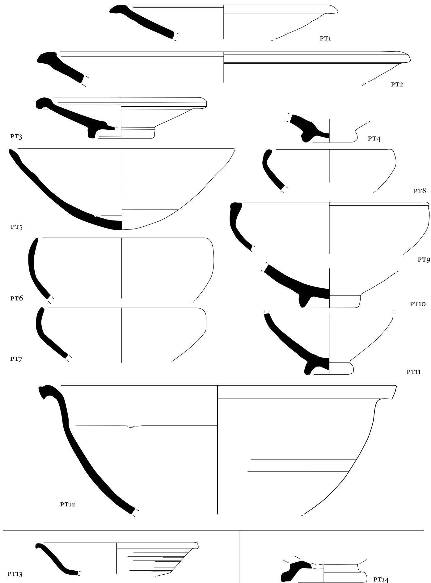
Plate 1. Group A. Local Hellenistic fine ware (PT1–12); Hellenistic fine gray ware (PT13); Eastern Sigillata A (PT14). Scale 1:2.
