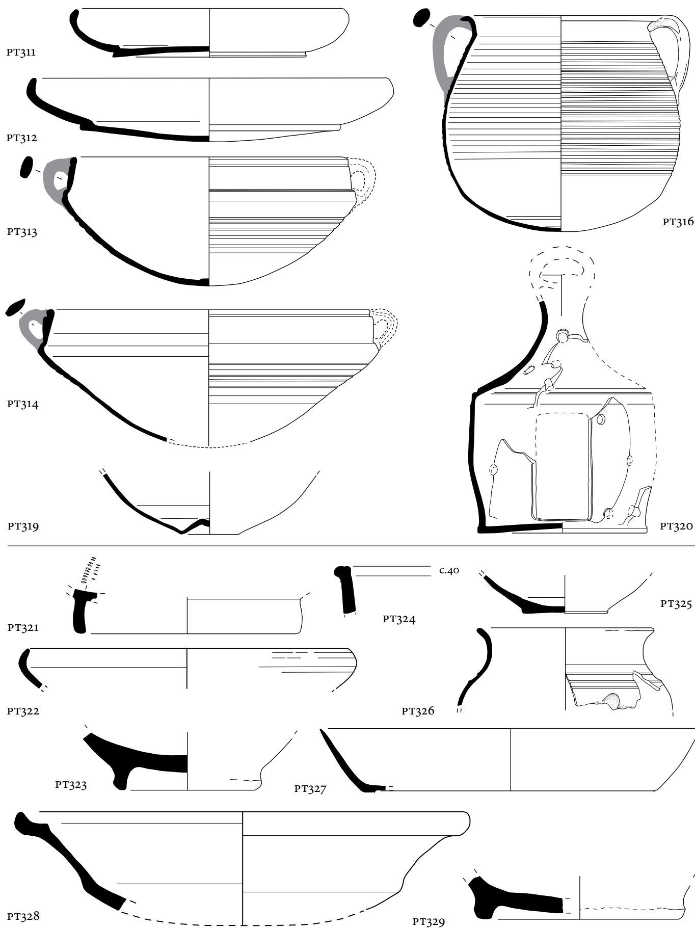
Plate 18. Group D. Group of cooking-ware vessels from context 2176 (PT311–320). Scale 1:3. BSP (PT321, 322); local Hellenistic fine ware (PT323); Italian Sigillata (PT324); thin-walled wares (PT325, 326); African Red Slip Ware (PT327); “Parthian” glazed ware (PT328, 329). Scale 1:2.
