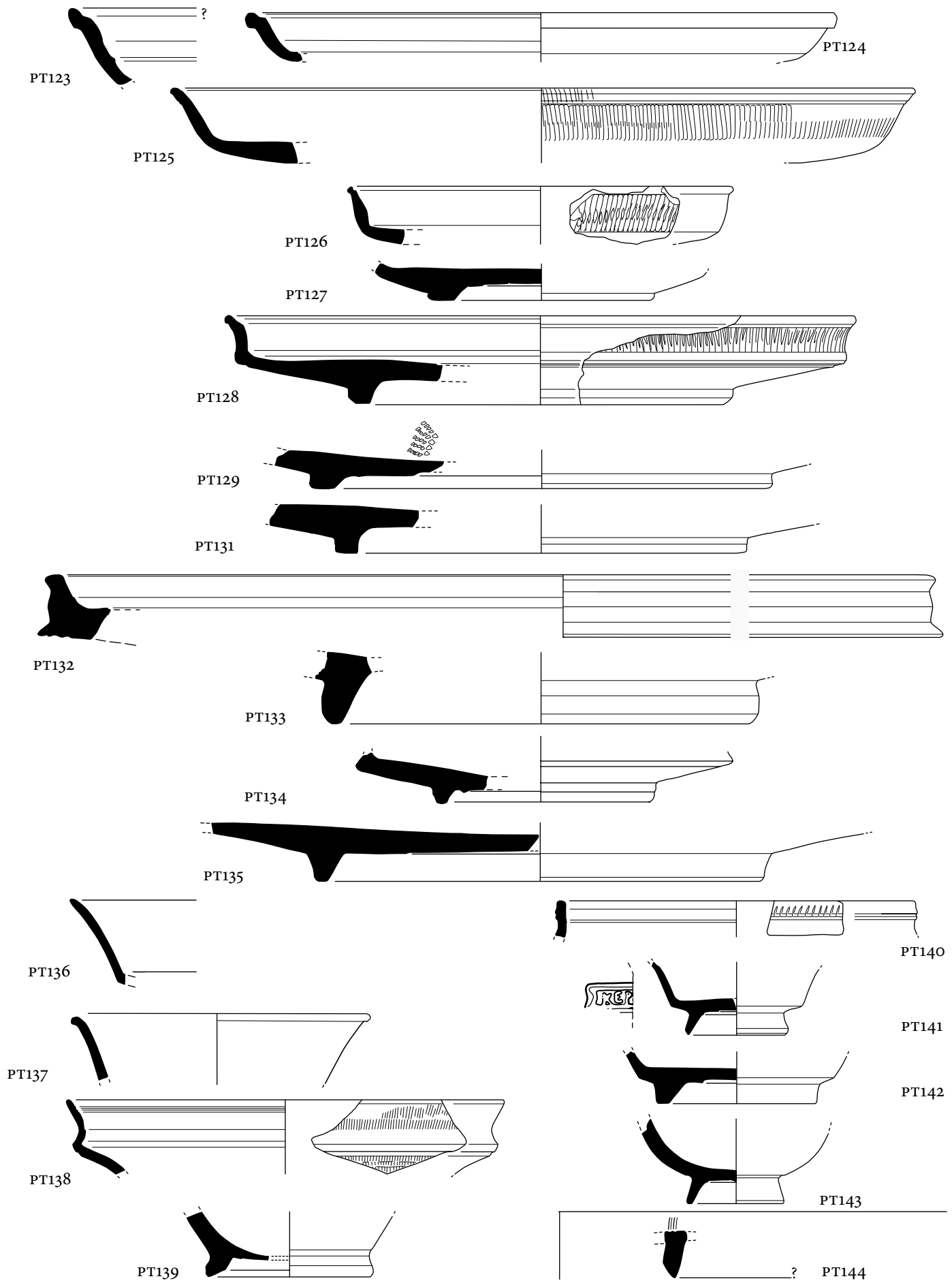
Plate 9. Group B. Eastern Sigillata A (PT123–143); Italian Sigillata (PT144). Scale 1:2 (stamp on PT141, 1:1).
