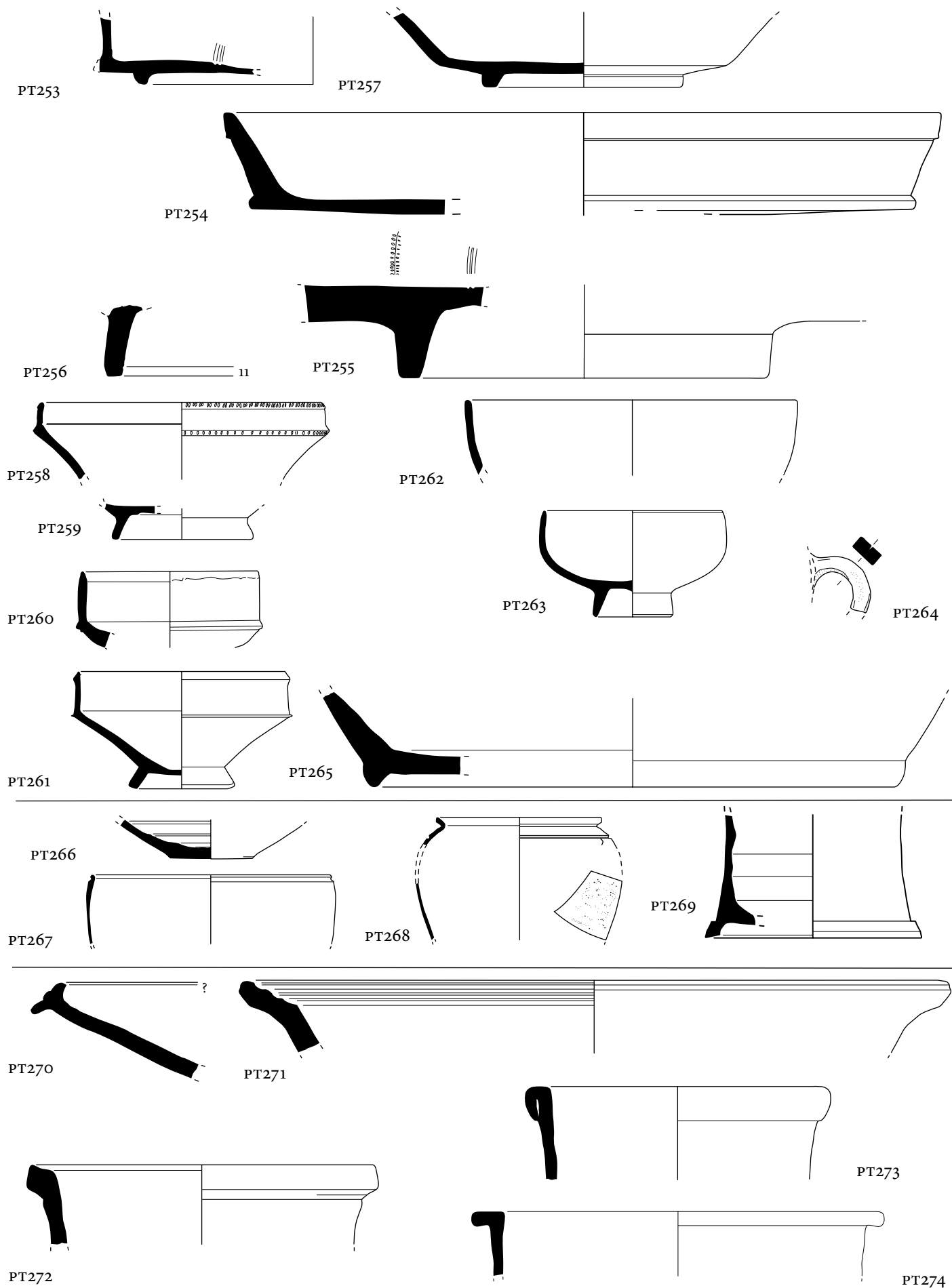
Plate 15. Group C. Eastern Sigillata A (PT253–265); thin-walled wares (PT266–268); miscellaneous fine ware (PT269). Scale 1:2. Buff wares 1–4 (PT270–274). Scale 1:3.
