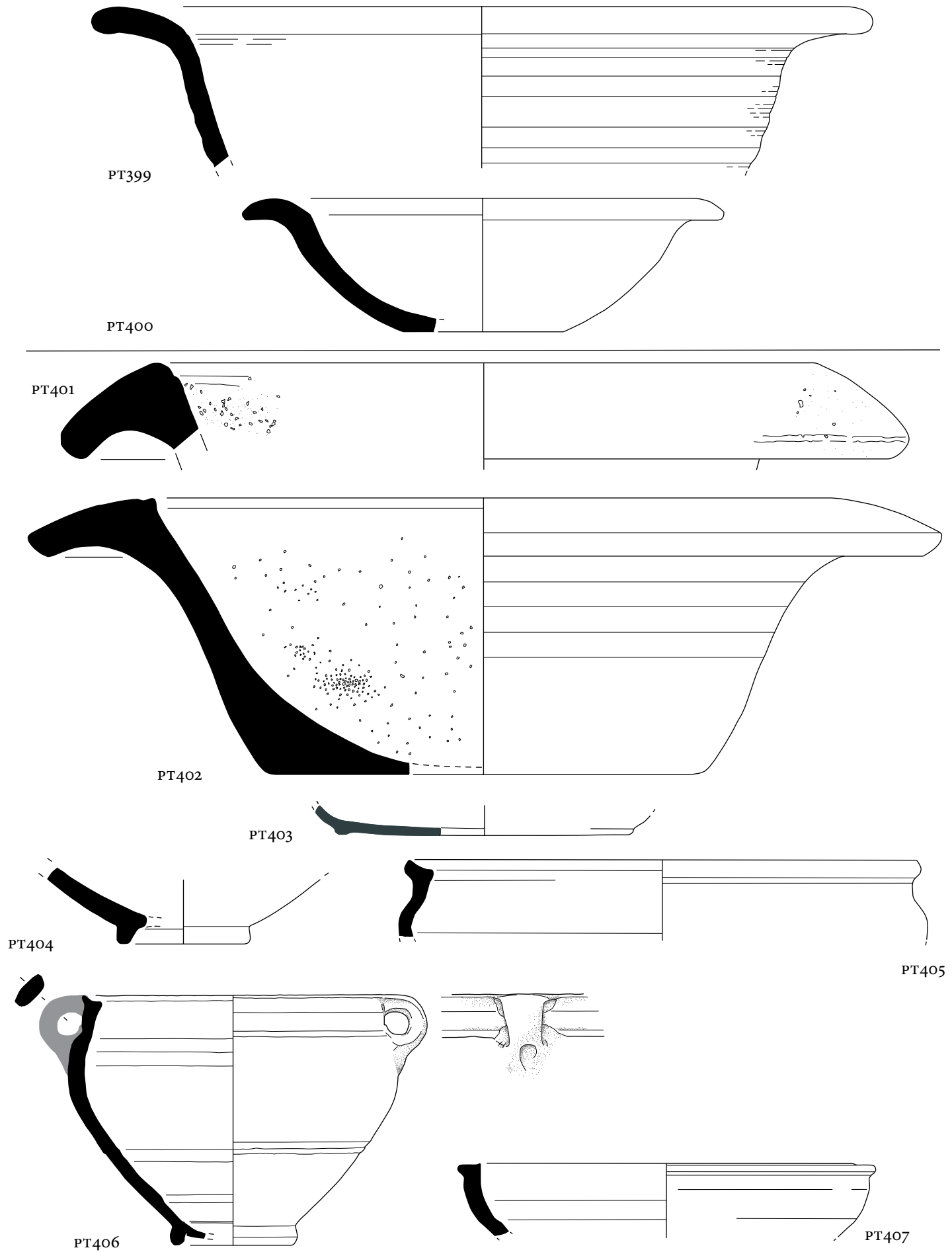
Plate 25. Group D. Buff ware 6 (PT399, 400); other buff wares (PT401–407). Scale 1:3.
