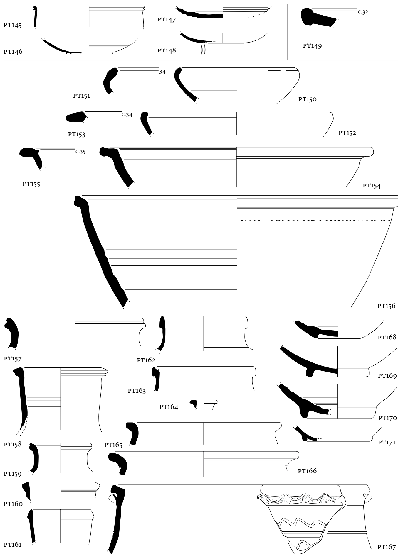
Plate 10. Group B. Thin-walled wares (PT145–148); African Red Slip Ware (PT149). Scale 1:2. Buff wares 1–4 (PT150–171). Scale 1:3.
