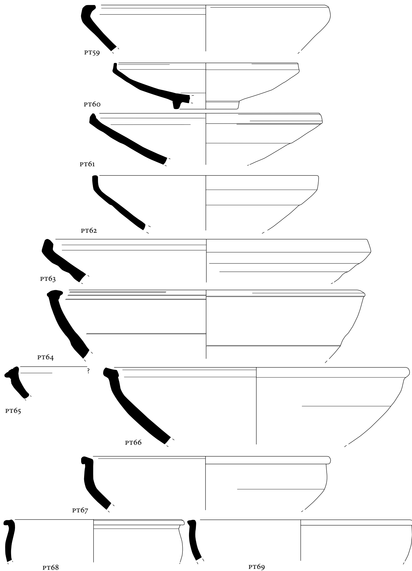
Plate 5. Group B. Local Hellenistic fine ware (PT59–69). Scale 1:2.
