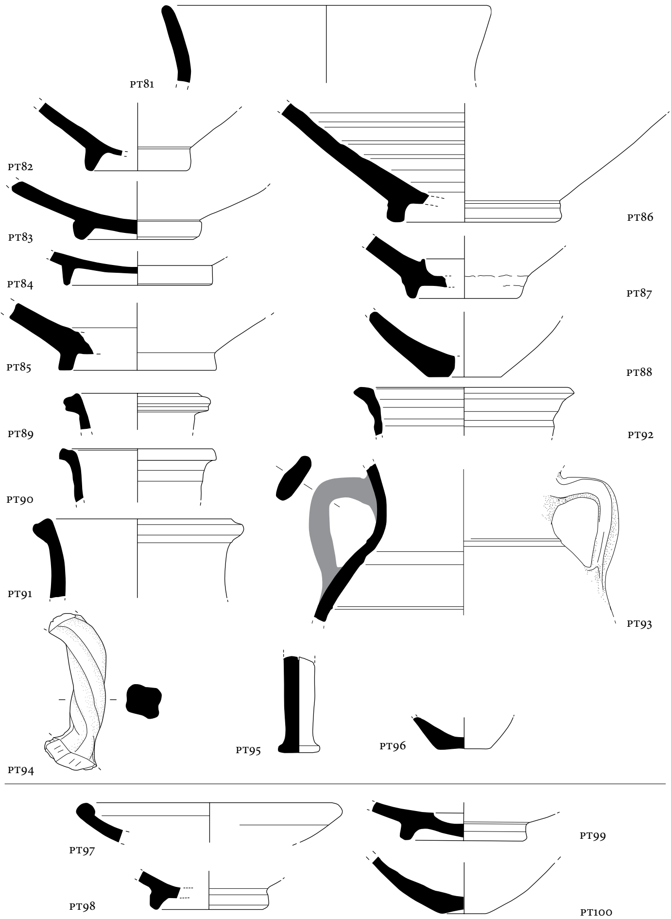
Plate 7. Group B. Local Hellenistic fine ware (PT81–96); miscellaneous Hellenistic fine wares (PT97–100). Scale 1:2.
