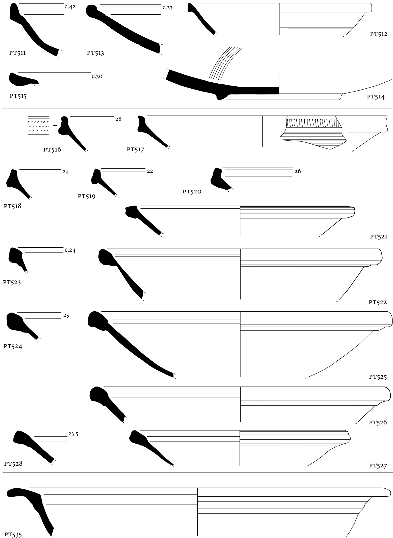
Plate 33. Group F. African Red Slip Ware (PT511–515); Phocaeian Red Slip Ware (PT516–528). Scale 1:2. Buff ware 1 (PT535). Scale 1:3.
