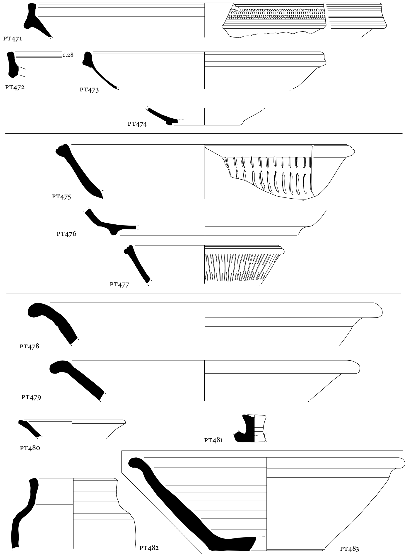
Plate 30. Group E. Phocaeen Red Slip Ware (PT471-474); Cypriot Red Slip Ware (PT475-477). Scale 1:2. Buff wares 1-3 (PT478-482); Buff ware 6 (PT483). Scale 1:3.
