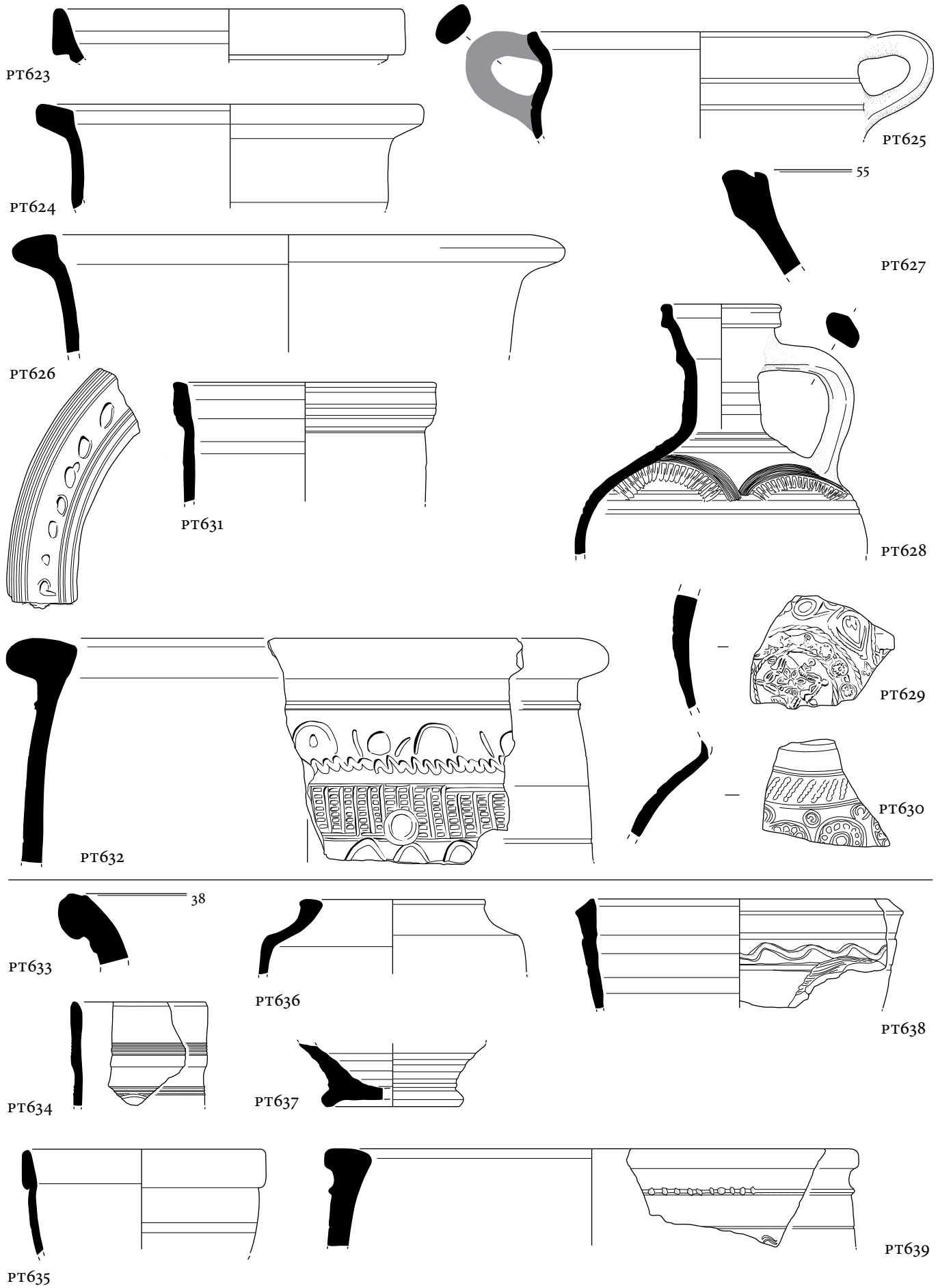
Plate 41. Group G. Buff ware 8 (PT623–632); Buff ware 10 (PT633–639). Scale 1:3 (PT629, 630, 1:2).
