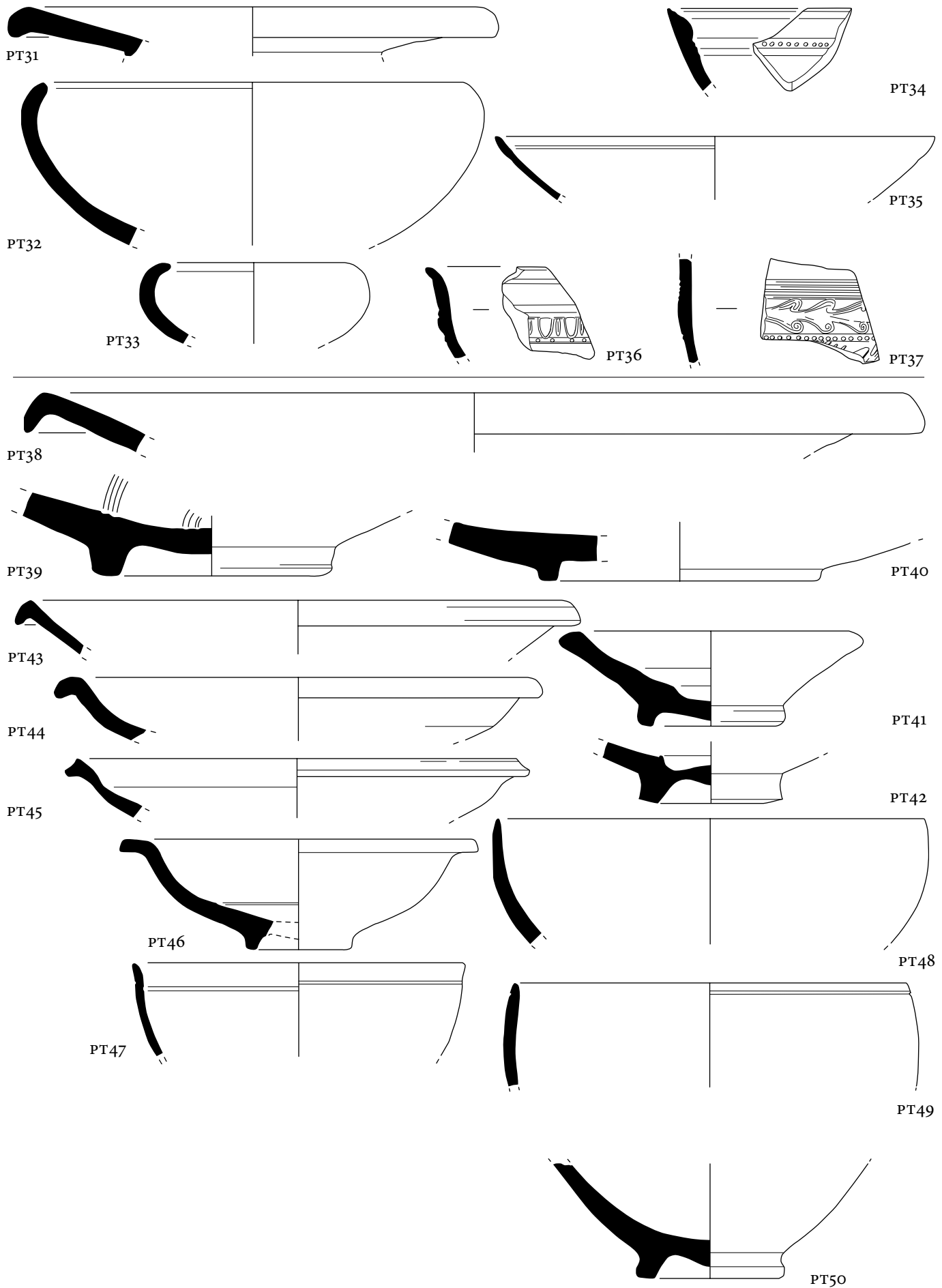
Plate 3. Group B. BSP (PT31–37); Local Hellenistic fine ware (PT38–50). Scale 1:2.
