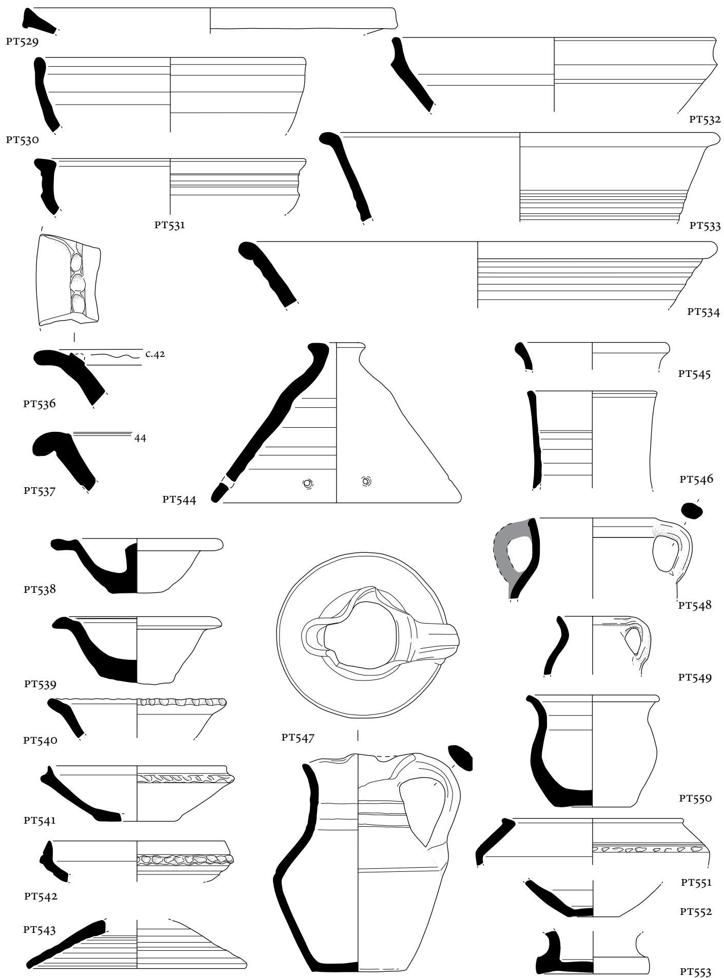
Plate 34. Group F. Buff wares 1-4 (PT529-534, 536-553). Scale 1:3.
